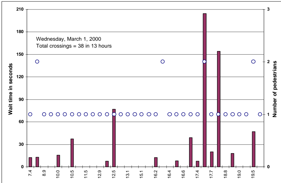
FIGURE 2. Pedestrian crossings and delays without in-pavement lights.
